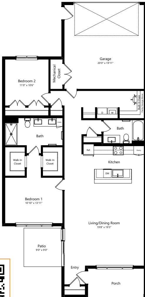
2D PLAN
