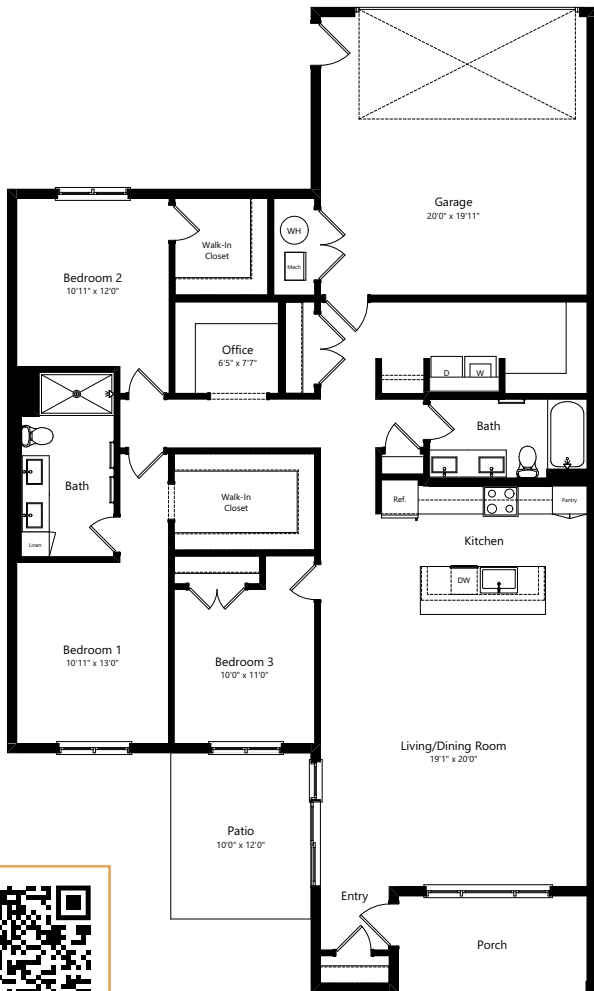
2D PLAN
