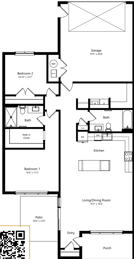
2D PLAN
